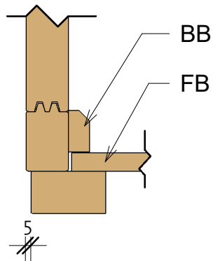
Floor Schedule
